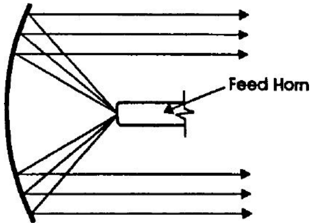
Prime-focus feed
