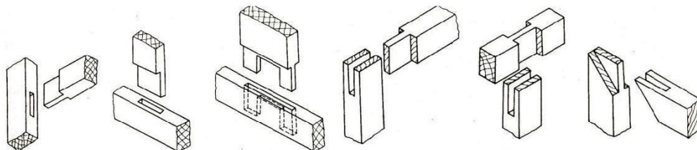
Bridle Joint
