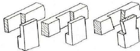
Lap joints
