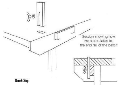
Bench Stop
