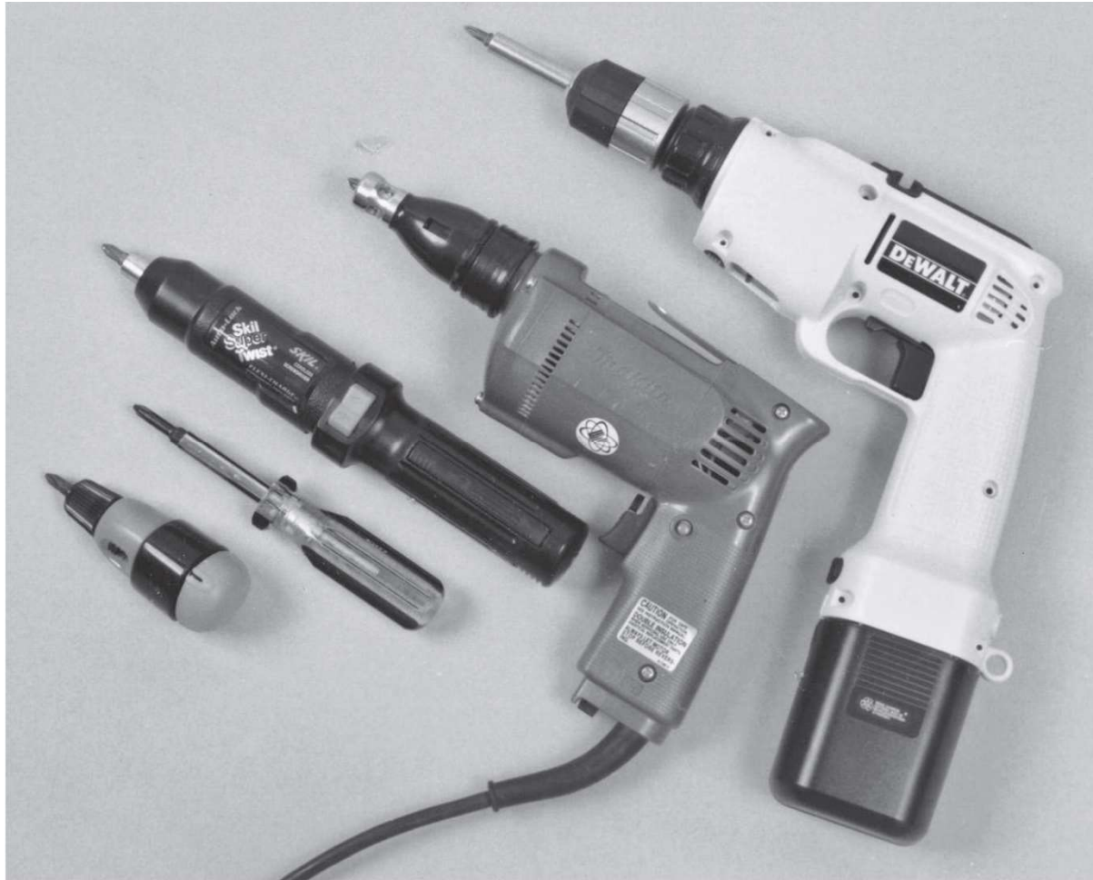
Figure 2.1: Existing products used to drive screws: manual screwdrivers, cordless screwdriver, screw gun, cordless drill with driver bit.
