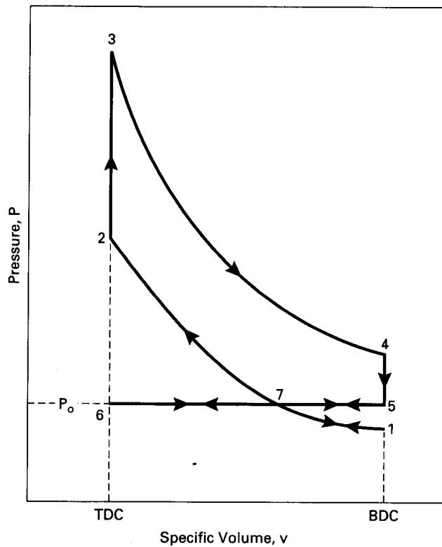
Figure 3-14 Air-standard Miller cycle for unthrottled naturally aspirated four-stroke cycle SI engine. If the engine has early intake valve closing, the cycle will be 6-7-1-7-2-3-4-5-6. If the engine has late intake valve closing, the cycle will be 6-7-5-7-2-3-4-5-7-6.
