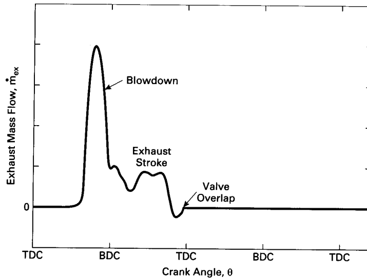
Figure 8-2 Exhaust gas flow out of cylinder through the exhaust valve(s), showing blowdown and exhaust stroke. Possible reverse flow back into the cylinder may occur during valve overlap. Adapted from [28].
