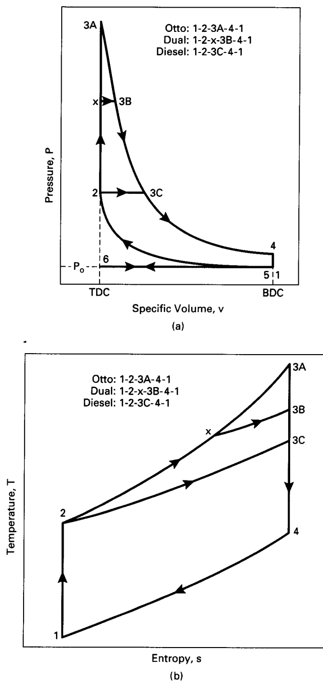
Figure 3-11 Comparison of air-standard Otto cycle, Dual cycle, and Diesel cycle. All engines have the same cylinder input conditions and same compression ratio.
